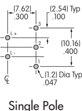
Single Pole
