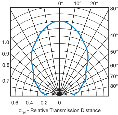
Fig. 11 - Horizontal Directivity
