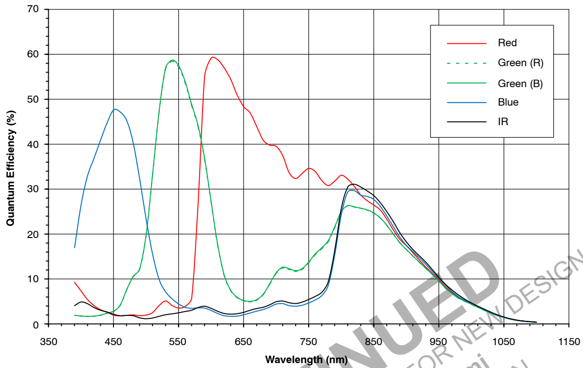
Figure 11. Quantum Efficiency - RGB-IR
