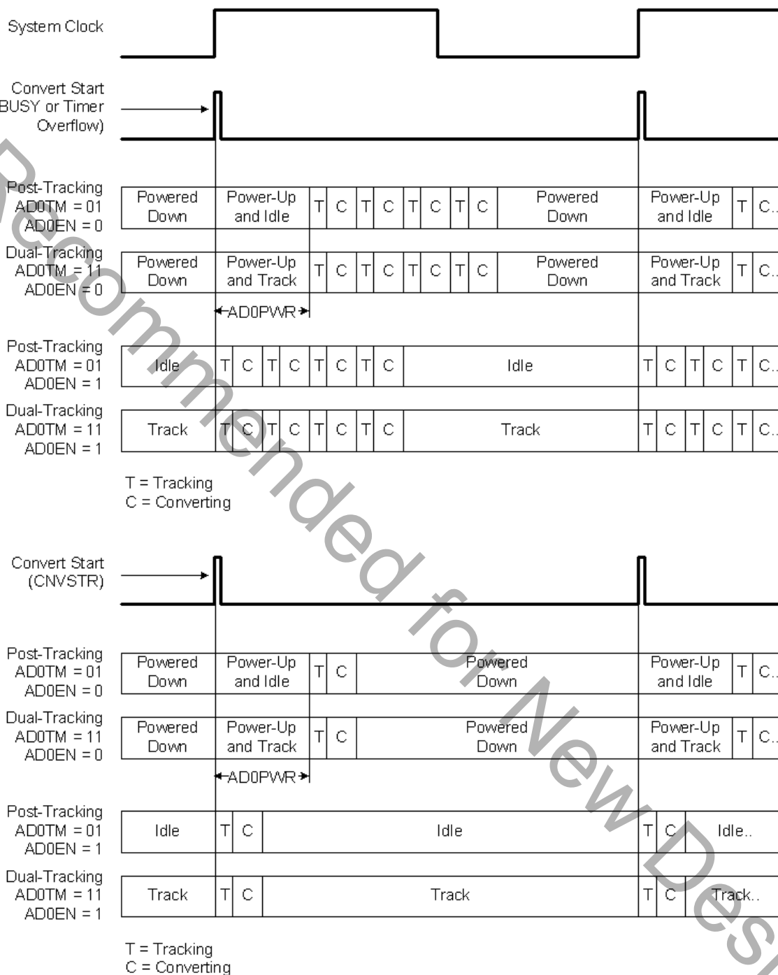
Figure 5.3. Burst Mode Tracking Example with Repeat Count Set to 4
