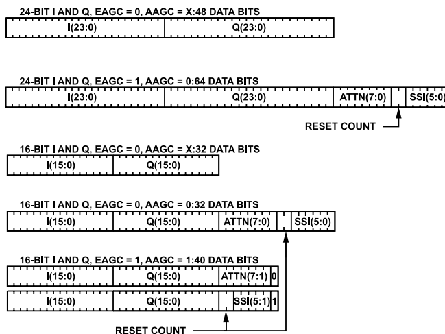
Figure 32. SSI Frame Structure
