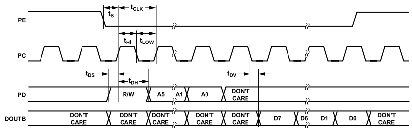
Figure 31. 4-Wire SPI Read Operation Timing
