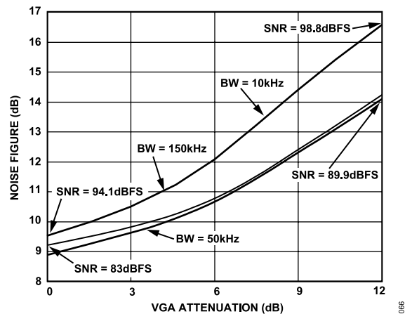
Figure 67. Nominal System Noise Figure and Peak SNR vs. AGCG Setting ( f_{IF} = 73.35 \text{ MHz} , f_{CLK} = 18 \text{ MSPS} , and 16-bit I/Q Data)
