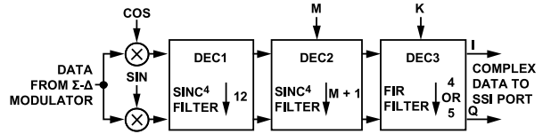
Figure 52. Decimation Filter Architecture
