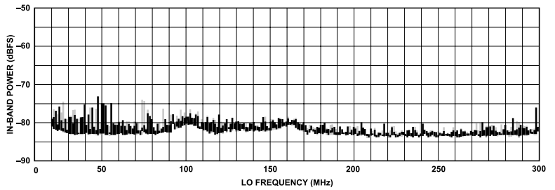
Figure 70. Same as Figure 69 Excluding LO Frequencies Known to Produce Large In-Band Spurs
