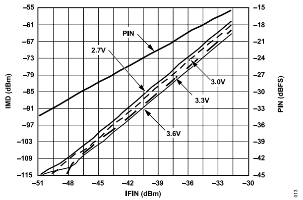
Figure 13. IMD vs. IFIN
