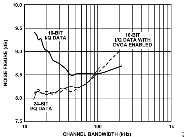
Figure 11. Noise Figure vs. Bandwidth (Minimum Attenuation, f_{CLK} = 13 MSPS)
