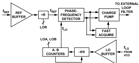
Figure 39. LO Synthesizer
