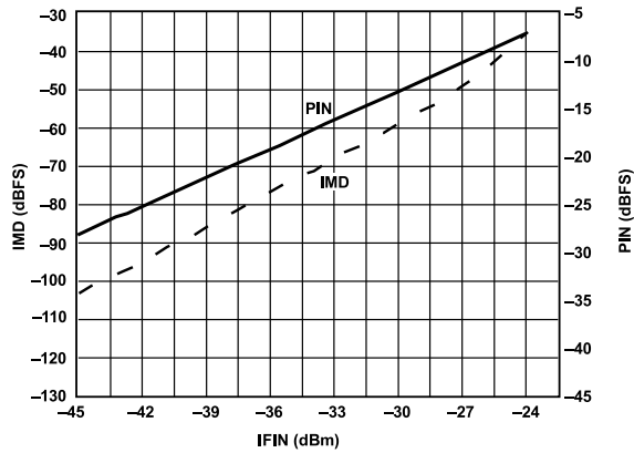
Figure 21. IMD vs. IFIN ( f_{CLK} = 26 MSPS)
