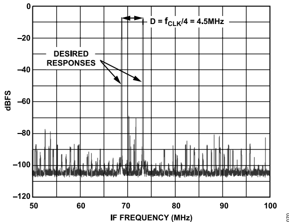
Figure 71. Response of AD9864 to a -20 dBm IF Input when f_{LO} = 71.1 MHz
