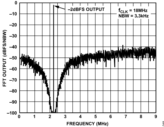
Figure 48. Measured Undecimated Spectral Output of \Sigma - \Delta Modulator ADC with f_{CLK} = 18 MSPS and Noise Bandwidth of 3.3 kHz
