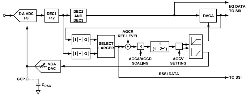
Figure 59. Functional Block Diagram of VGA and AGC
