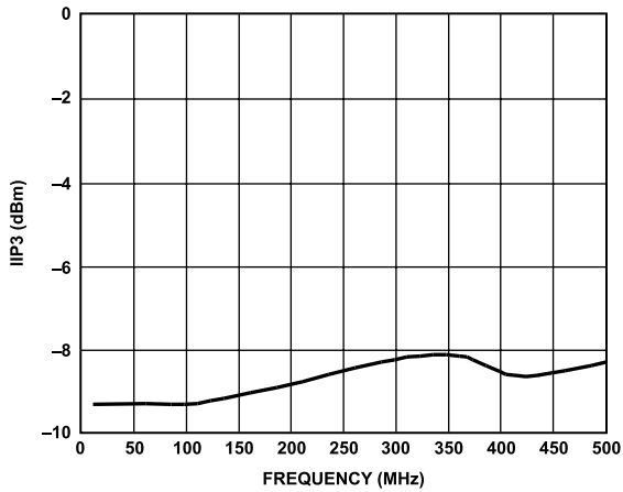
Figure 25. Input IIP3 vs. Frequency ( f_{CLK} = 18 MSPS)
