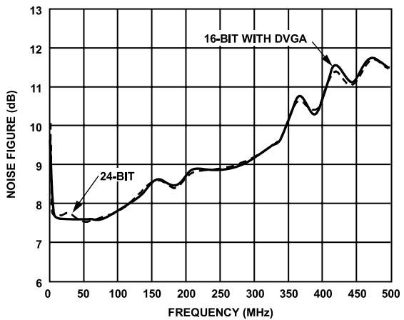
Figure 22. Noise Figure vs. Frequency (Minimum Attenuation, f_{CLK} = 26 MSPS, BW = 10 kHz)
