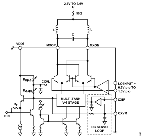
Figure 44. Simplified Schematic of AD9864 LNA/Mixer
