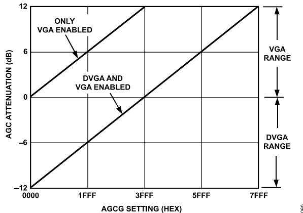
Figure 60. AGC Gain Range Characteristics vs. AGCG Register Setting With and Without DVGA Enabled
