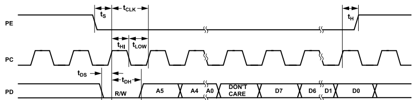
Figure 29. SPI Write Operation Timing
