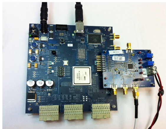
Figure 77. Evaluation Board Platform
