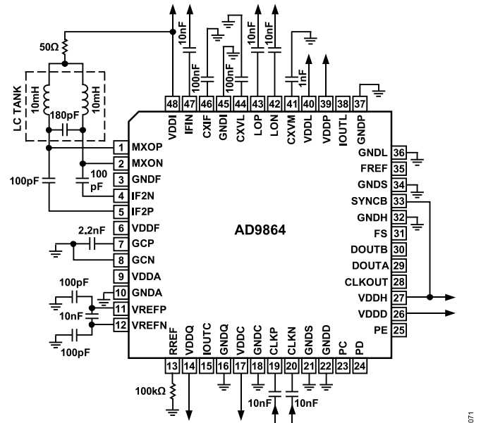
Figure 72. Example Circuit Showing Recommended Component Values
