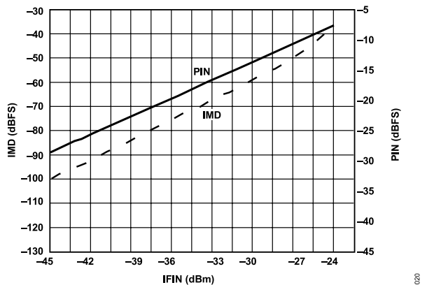
Figure 20. IMD vs. IFIN ( f_{CLK} = 18 MSPS)
