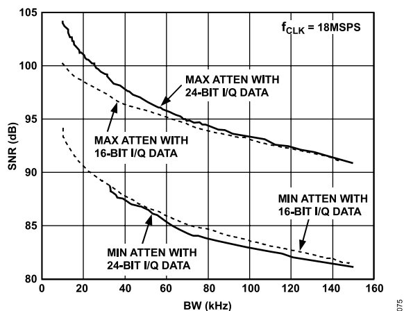
Figure 76. Hung Mixer SNR vs. BW and VGA
