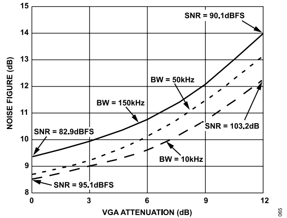
Figure 66. Nominal System Noise Figure and Peak SNR vs. AGCG Setting ( f_{IF} = 73.35 \text{ MHz} , f_{CLK} = 18 \text{ MSPS} , and 24-bit I/Q Data)
