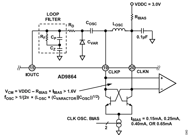
Figure 41. External Loop Filter, Varactor, and LC Tank Required to Realize a Complete Clock Synthesizer
