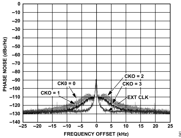
Figure 42. CLK Phase Noise vs. I_{BIAS} Setting (CKO); IF = 73.35 MHz, IF = 71.1 MHz, I_{FIN} = -31\text{ dBm} , f_{CLK} = 18\text{ MHz} , f_{REF} = 16.8\text{ MHz} ; CLK SYN Settings: CKI = 7 , CLR = 56 , and CLN = 60 with f_{REF} = 300\text{ kHz}
