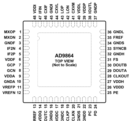
Figure 2. 48-Lead LFCSP Pin Configuration
