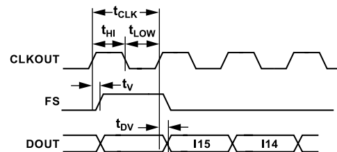
Figure 34. SSI Timing Parameters for SSI Timing
