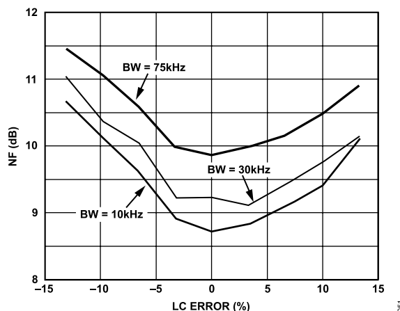
Figure 51. Typical Noise Figure Degradation from L and C Component Drift ( f_{\text{CLK}} = 18 MSPS, f_{\text{IF}} = 73.3501 MHz)
