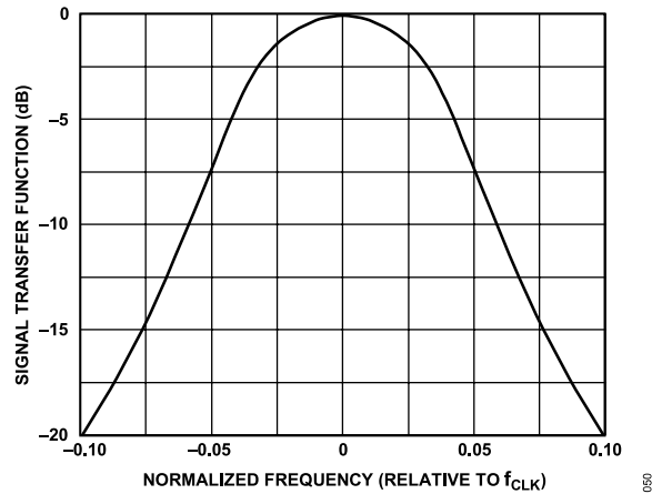
Figure 50. Magnitude of the Signal Transfer Function of the ADC near f_{CLK}/8
