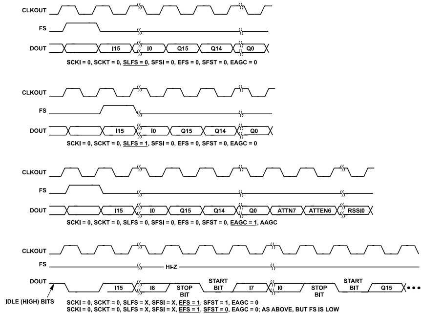
Figure 33. SSI Timing for Several SSICRA Settings with 16-Bit I/Q Data
