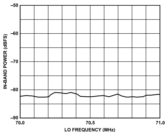
Figure 68. Expanded View from 70 MHz to 71 MHz
