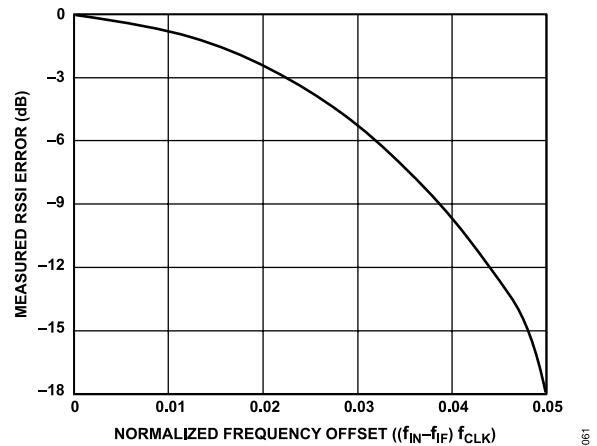
Figure 61. Normalized RSSI Error vs. Normalized IF Frequency Offset
