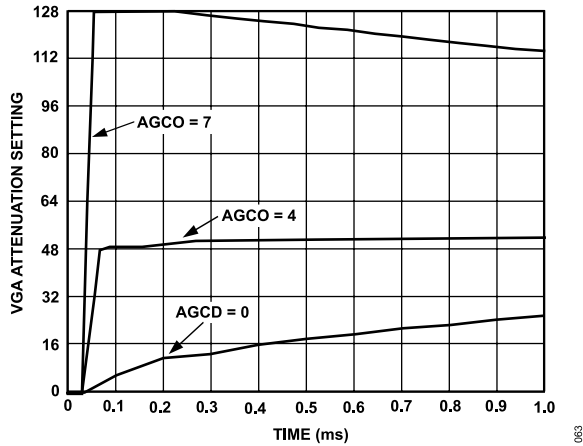
Figure 63. AGC Response for Different AGCO Settings with f_{CLK} = 18 \text{ MSPS} , f_{CLKOUT} = 300 \text{ kSPS} , Decimate by 60 and AGCA = AGCD = 0
