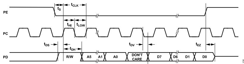
Figure 30. 3-Wire SPI Read Operation Timing
