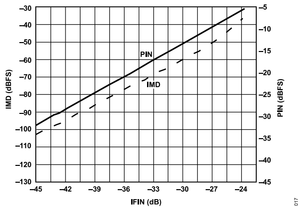
Figure 17. IMD vs. IFIN ( f_{CLK} = 13 MSPS)
