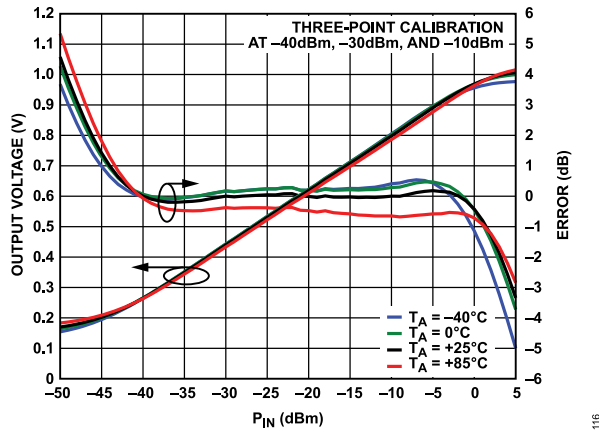
Figure 16. V_{LOG} and Log Conformance Error vs. P_{IN} over Temperature at 900 MHz
