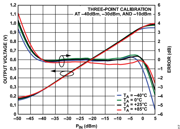
Figure 17. V_{LOG} and Log Conformance Error vs. P_{IN} over Temperature at 1900 MHz
