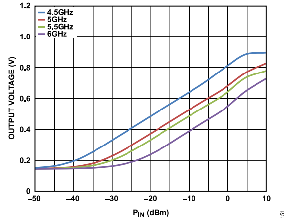
Figure 50. V_{\text{LOG}} vs. P_{\text{IN}} over Frequency (4.5 GHz to 6 GHz)
