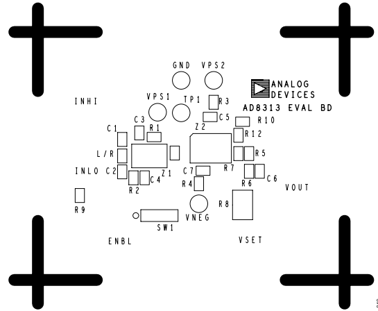
Figure 43. Signal Layer Silkscreen
