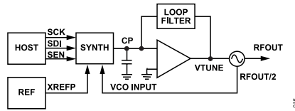
Figure 16. Typical Application Diagram
