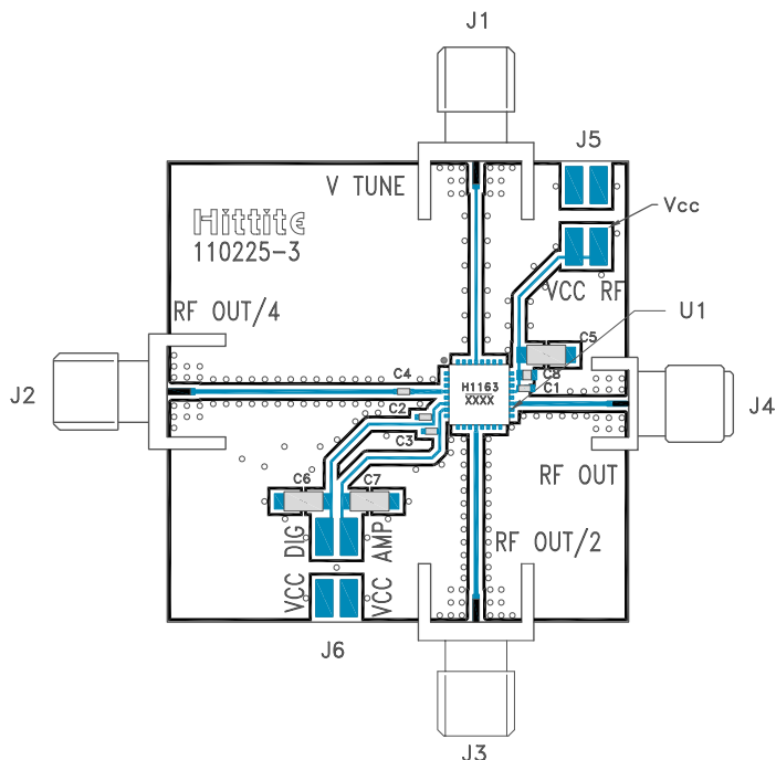
Figure 17. Evaluation PCB
