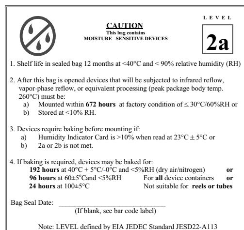
Fig. 14 - Example of JESD22-A112 level 2a label
