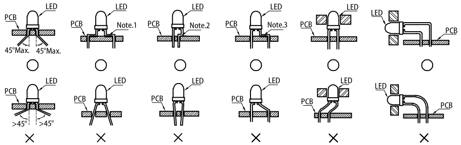
" ○ " Correct mounting method " × " Incorrect mounting method
