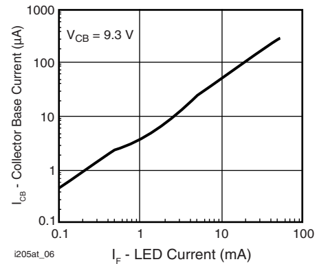
Fig. 6 - Collector Emitter Photocurrent vs. LED Current
