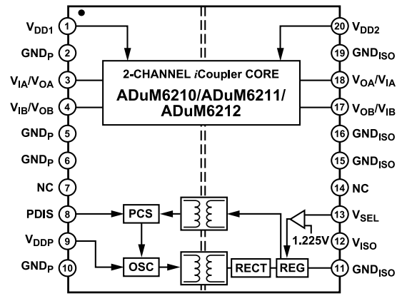
Figure 1. ADuM6210/ADuM6211/ADuM6212
