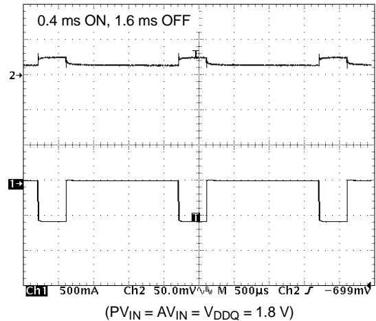
Upper Trace: VTT Output Waveform, 50 mV/Division, AC Coupled Lower Trace: Loading Current, IVTT, 500 mA/Division (P VIN = A VIN = V DDQ = 1.8 V)
