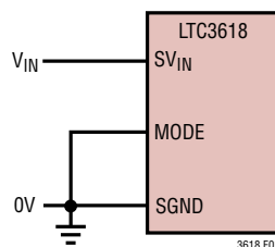
1b. Forced Continuous Mode
