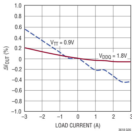
V_{\text{OUT}} Load Regulation
