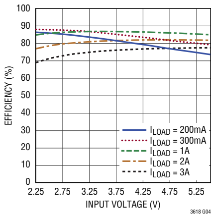
Efficiency vs Input Voltage V_{\text{TT}} = 0.9\text{V}
