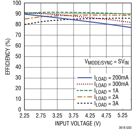
Efficiency vs Input Voltage V_{\text{DDQ}} = 1.8\text{V}
