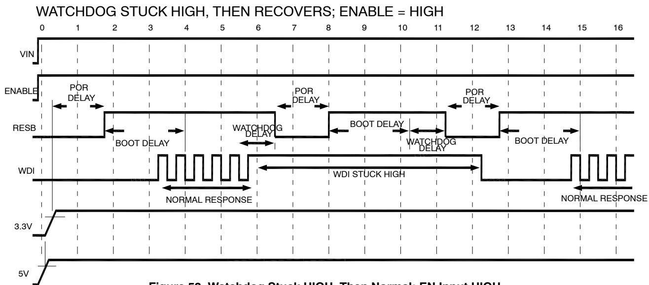
Figure 53. Watchdog Stuck HIGH, Then Normal; EN Input HIGH
