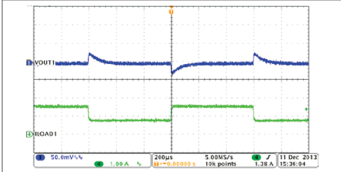
Figure 8-15. Buck1, Load Transient, 0.75 to 1.5 A SR = 0.25 A/µs
