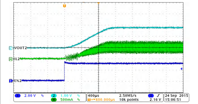
Figure 8-30. PWM Mode, Buck2, Soft-Start with Full Load
