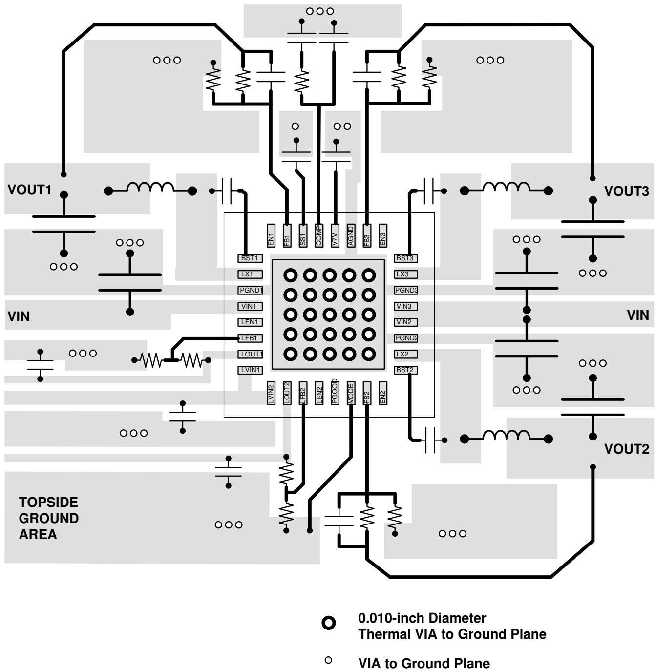
Figure 8-37. PCB Layout
