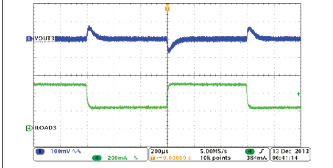
Figure 8-19. Buck3, Load Transient, 0.25 to 0.5 A SR = 0.25 A/µs
