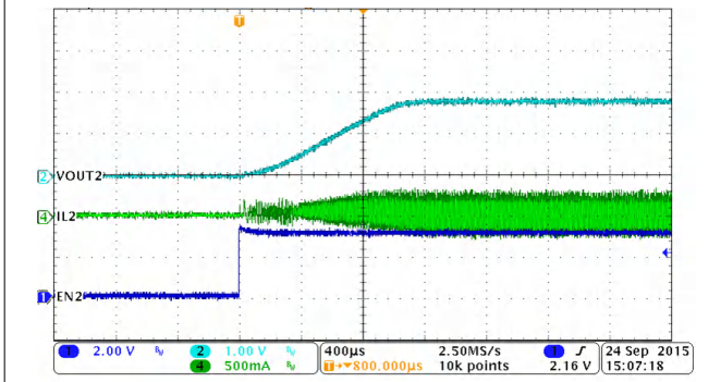
Figure 8-29. PWM Mode, Buck2, Soft-Start with No Load
