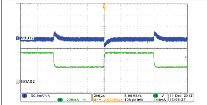
Figure 8-17. Buck2, Load Transient, 0.25 to 0.5 A SR = 0.25 A/µs
