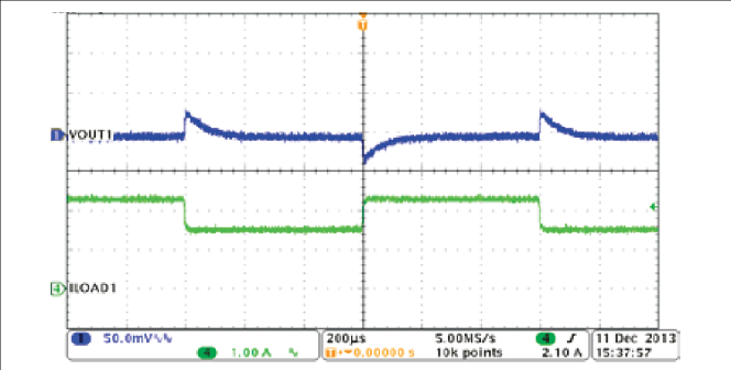
Figure 8-16. Buck1, Load Transient, 1.5 to 2.25 A SR = 0.25 A/µs
