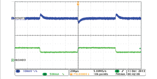
Figure 8-20. Buck3, Load Transient, 0.5 to 0.75 A SR = 0.25A/µs
