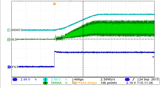
Figure 8-32. PWM Mode, Buck3, Soft-Start with Full Load
