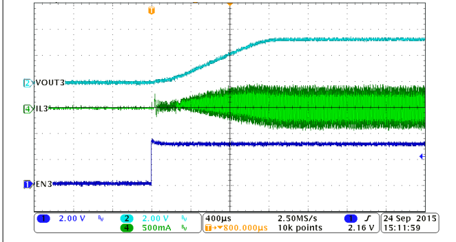
Figure 8-31. PWM Mode, Buck3, Soft-Start with No Load
