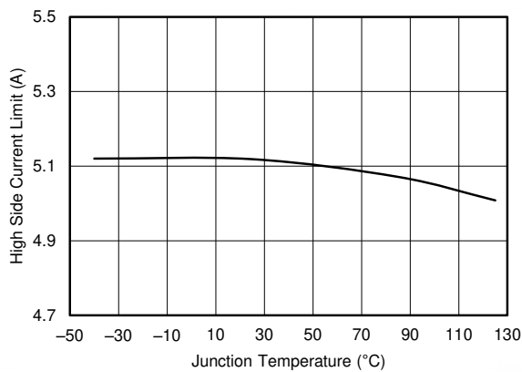
Figure 6-21. Buck1 High-Side Current Limit vs Temperature
