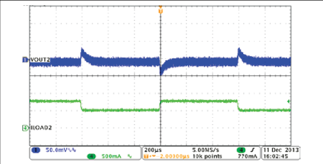
Figure 8-18. Buck2, Load Transient, 0.5 to 0.75 A SR = 0.25A/µs
