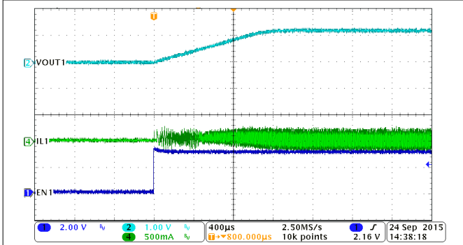
Figure 8-27. PWM Mode, Buck1, Soft-Start with No Load
