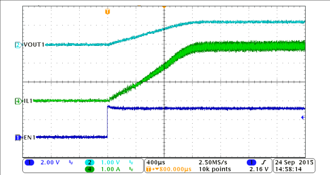
Figure 8-28. PWM Mode, Buck1, Soft-Start with Full Load
