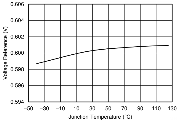
Figure 6-13. Voltage Reference vs Temperature
