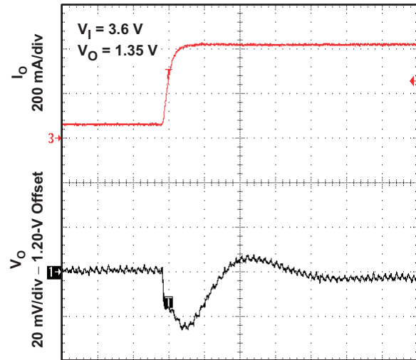
LOAD TRANSIENT: 50 mA / 400 mA PWM OPERATION
