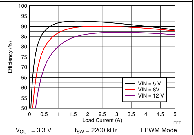
Figure 30. LM73605 Efficiency
