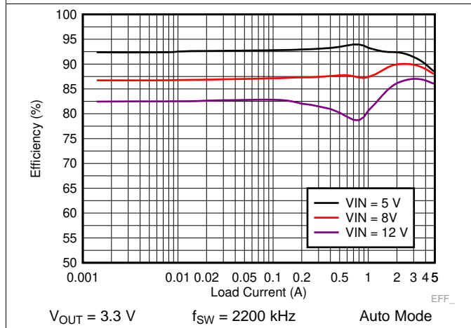
Figure 29. LM73605 Efficiency
