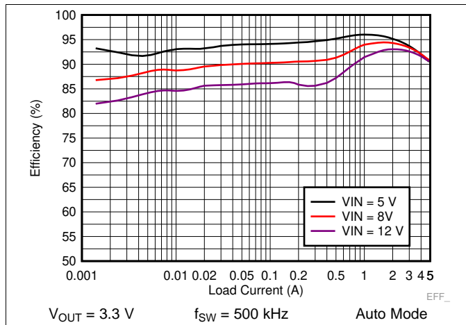
Figure 27. LM73605 Efficiency
