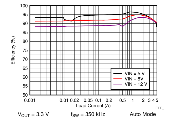
Figure 31. LM73605 Efficiency
