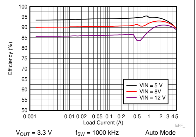
Figure 32. LM73605 Efficiency
