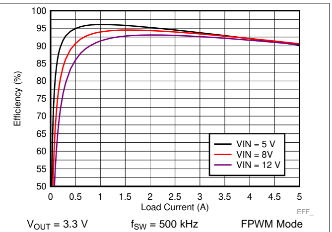
Figure 28. LM73605 Efficiency
