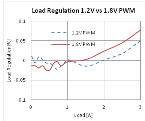
Load Regulation: % of V_{OUT} vs. I_{OUT} (PWM)
