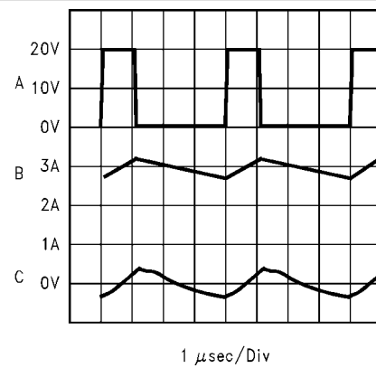
Continuous Mode Switching Waveforms V_{IN} = 20V, V_{OUT} = 5V, I_{LOAD} = 3A, L = 33\mu H, C_{OUT} = 200\mu F, C_{OUTESR} = 26m\Omega A: V_{SW} Pin Voltage, 10 V/div. B: Inductor Current, 1 A/div C: Output Ripple Voltage, 20 mV/div AC-Coupled
