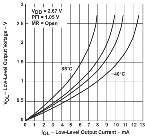
Figure 7-8. Low-Level Output Voltage vs Low-Level Output Current
