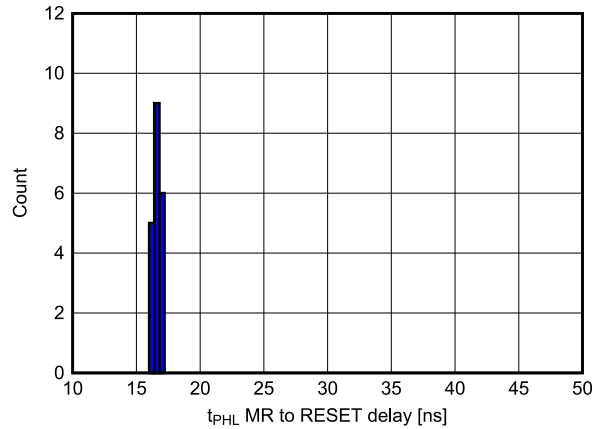
Figure 7-15. \overline{\text{MR}} to RESET ( t_{\text{PHL}} ) Delay Histogram for TPS3705-33 Devices at -40°C (Unit Count = 20)
