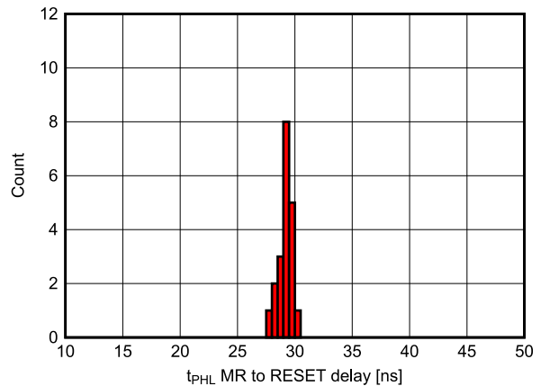
Figure 7-17. \overline{\text{MR}} to RESET ( t_{\text{PHL}} ) Delay Histogram for TPS3705-33 Devices at 125°C (Unit Count = 20)
