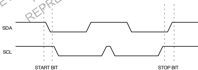
Figure 4. Start/Stop Timing
