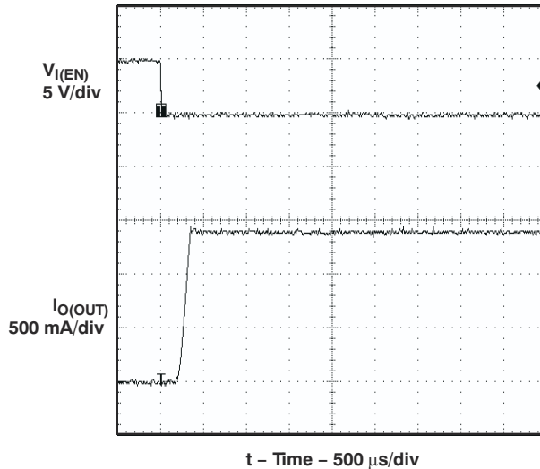
Figure 6-6. Short-Circuit Current, Device Enabled Into Short
