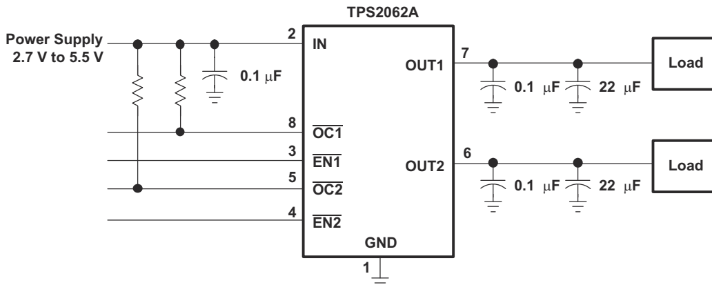
Figure 8-1. Typical Application
