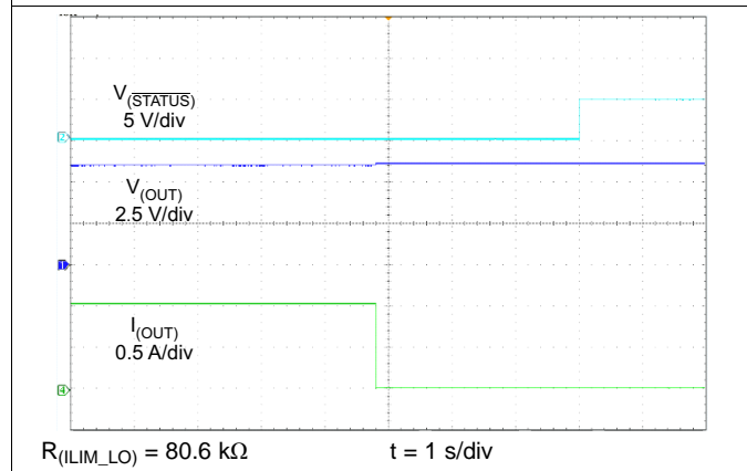
Figure 28. Load Detection Reset Time
