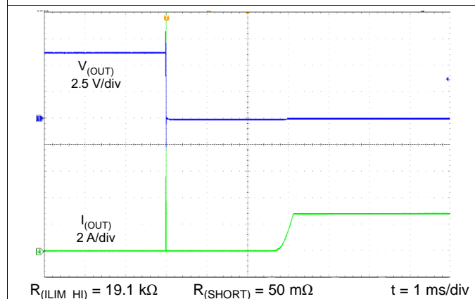
Figure 26. Hot Short
