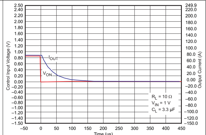
Figure 51. t_{OFF} Response
