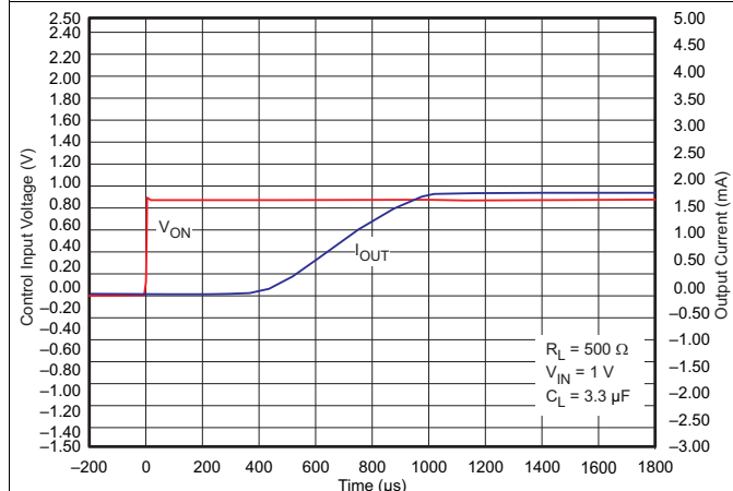
Figure 50. t_{ON} Response
