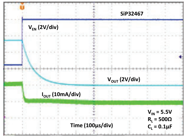
Fig. 31 - Turn-off Time
