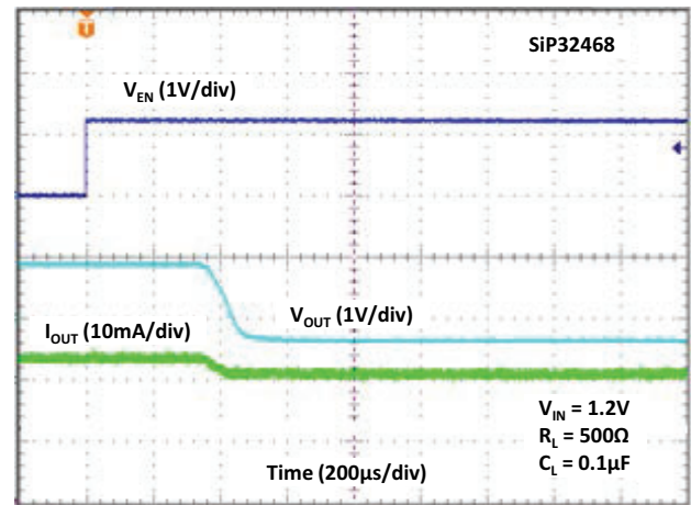
Fig. 32 - Turn-off Time
