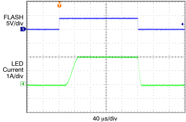
Figure 16. FLASH Transient Response
