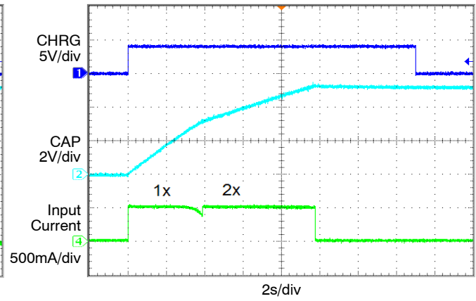
Figure 14. Charge Cycle, 500 mA Input Current
