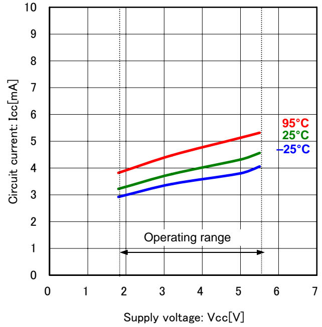
Fig.4 Circuit current STB
