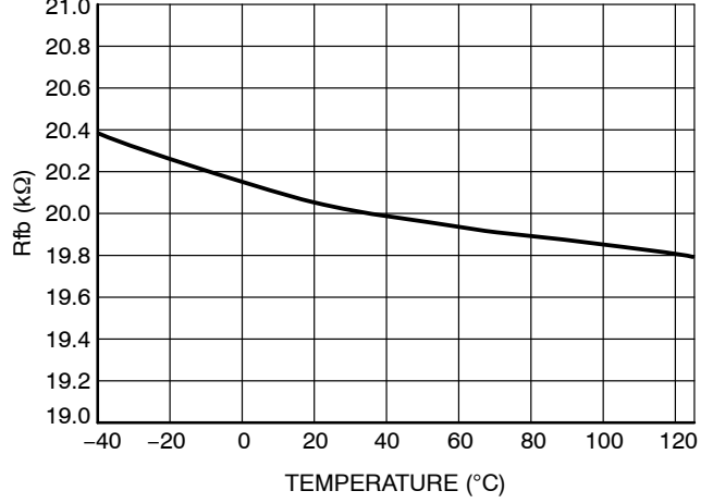
Figure 25. R_{FB} vs. Junction Temperature
