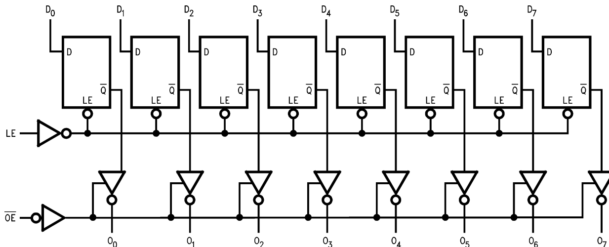
Figure 2. Logic Diagram
