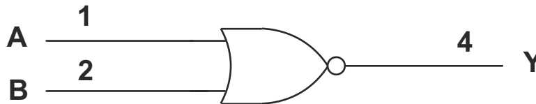
Figure 8-1. Logic Diagram
