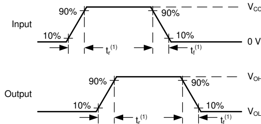
Figure 5-3. Voltage Waveforms, Input and Output Transition Times
