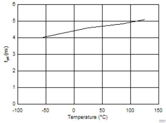
Figure 5-1. t pd vs Temperature at 3.3-V V CC
