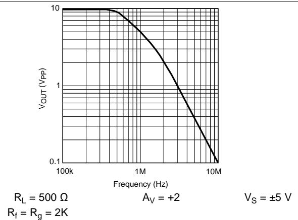
Figure 6. Output Swing vs. Frequency
