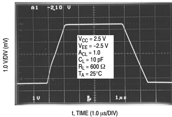
Figure 8. Slew Rate
