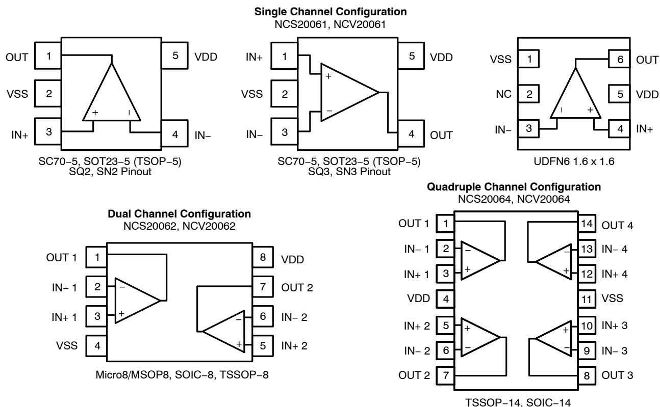
Figure 1. Pin Connections
