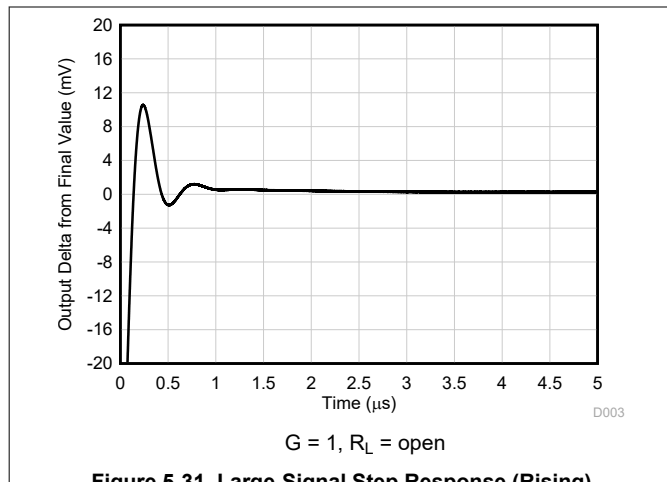
Figure 5-31. Large-Signal Step Response (Rising)
