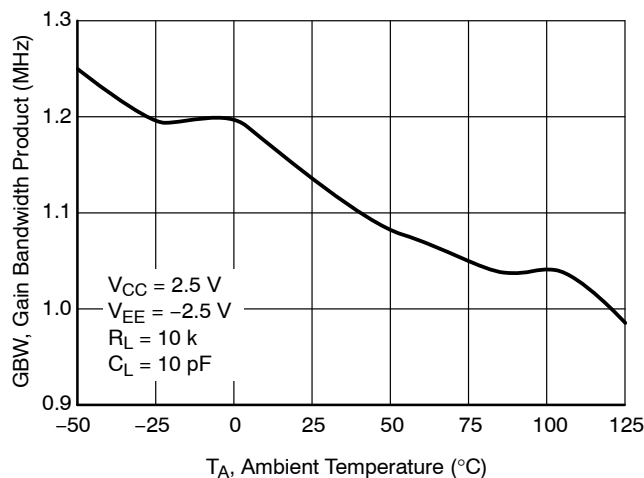
Figure 19. Gain Bandwidth Product vs. Temperature
