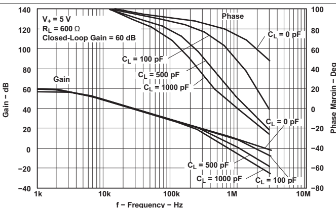
( C_L = 0 \text{ pF}, 100 \text{ pF}, 500 \text{ pF}, 1000 \text{ pF} ) Figure 24. Gain and Phase Margin vs Frequency
