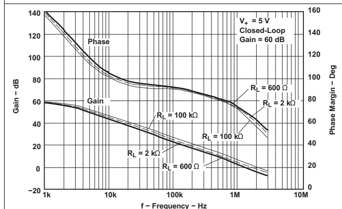
( R_L = 600 \Omega, 2 \text{ k}\Omega, 100 \text{ k}\Omega ) Figure 23. Gain and Phase Margin vs Frequency
