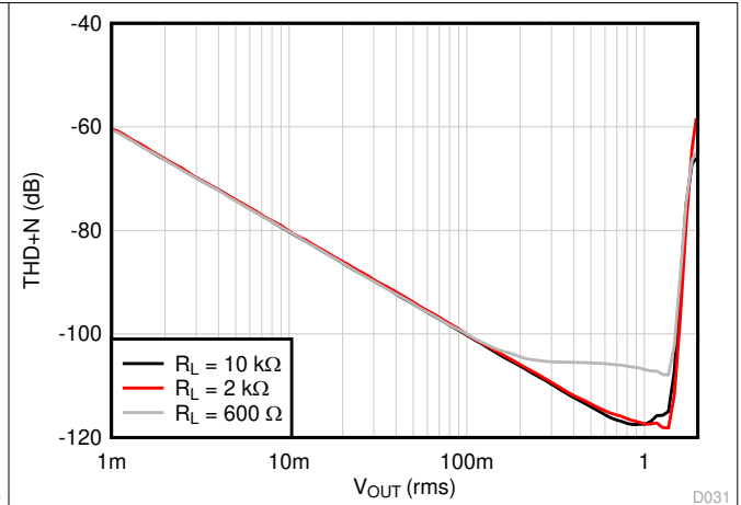
Figure 7-70. THD + N vs Amplitude
