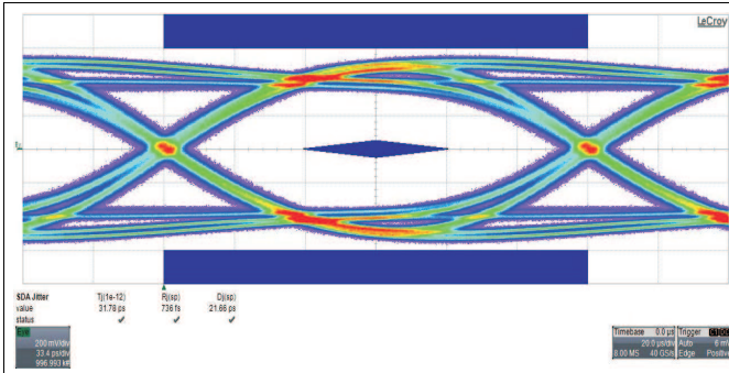
Figure 21. DE = 0 dB, EQ = 7 dB, Input = 12 Inches, Output = 8 Inches
