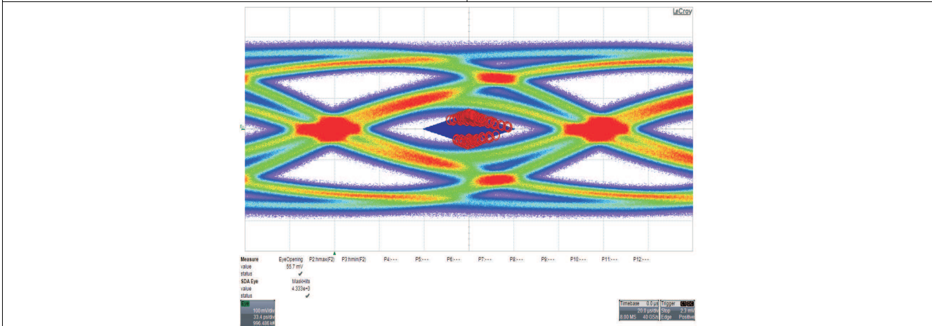
Figure 20. DE = 0 dB, EQ = 7 dB, Input = 12 inches, Output = 20 inches + 3-m Cable
