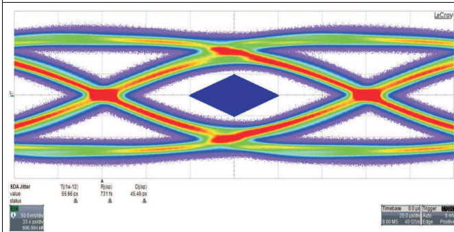
Figure 25. DE = -5 dB, EQ = 7 dB, Input = 12 Inches, Output = 40 Inches
