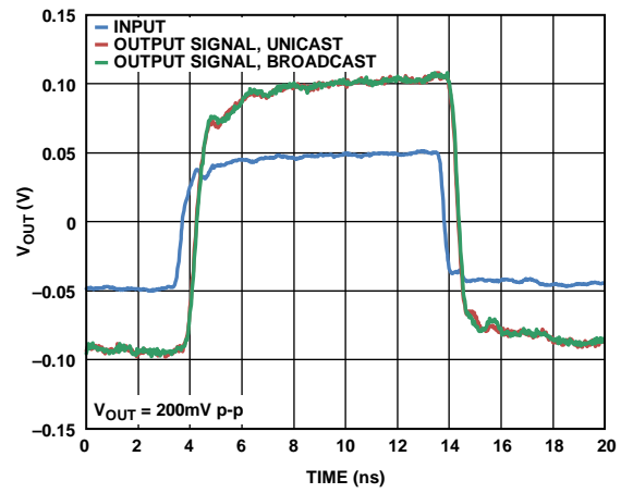
Figure 17. ADV3225 Small Signal Pulse Response
