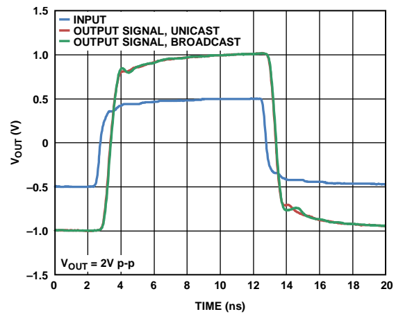
Figure 18. ADV3225 Large Signal Pulse Response
