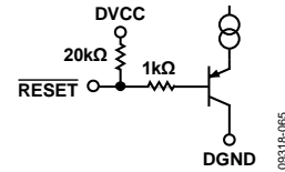
Figure 63. Reset Input
