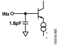
Figure 58. Analog Input
