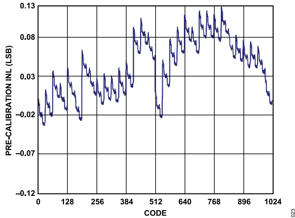
Figure 25. AD9715 Precalibration INL at 3.3 V
