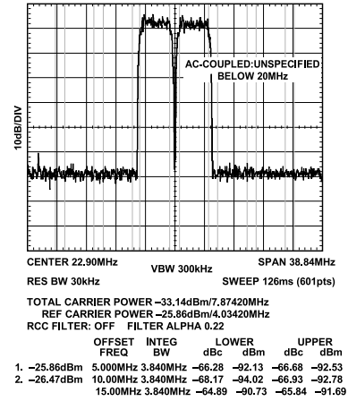
Figure 75. AD9717 Two-Carrier ACLR, 3.3 V
