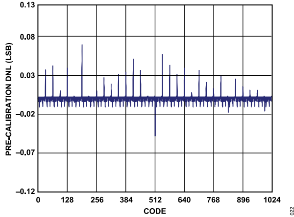
Figure 24. AD9715 Precalibration DNL at 1.8 V
