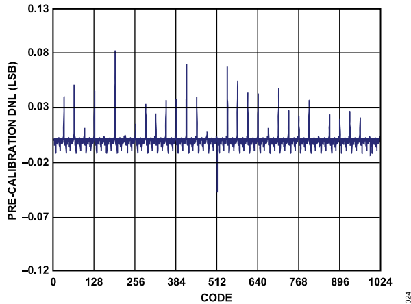
Figure 26. AD9715 Precalibration DNL at 3.3 V
