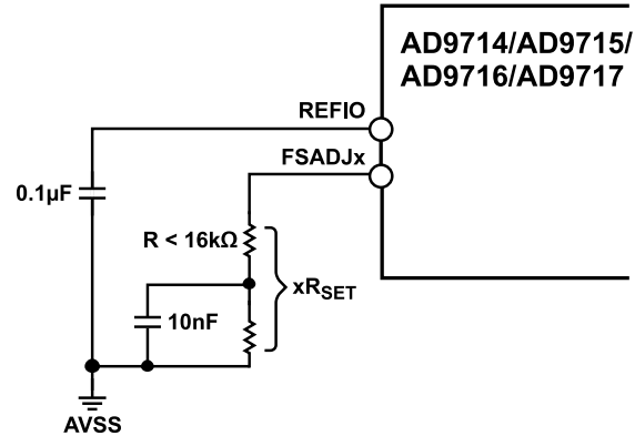
Figure 98. xR_{SET} Configuration for Values > 16 \text{ k}\Omega
