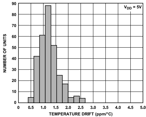
Figure 6. Reference Output Temperature Drift Histogram
