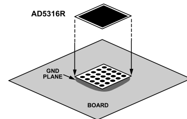
Figure 50. Paddle Connection to Board
