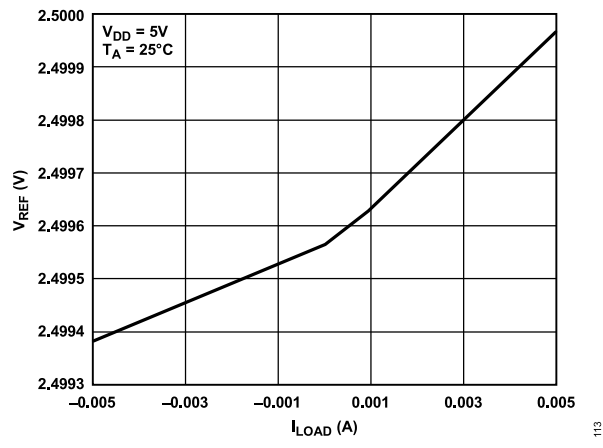
Figure 9. V_{REF} vs. Load Current ( I_{LOAD} )
