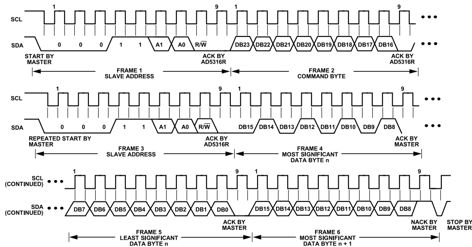
Figure 43. I 2 C Read Operation
