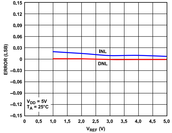
Figure 14. INL Error and DNL Error vs. V_{REF}
