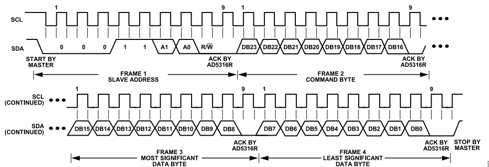
Figure 42. I 2 C Write Operation
