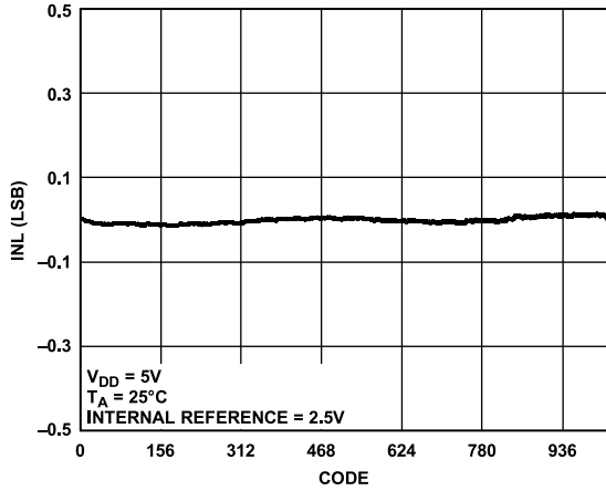
Figure 11. INL vs. Code
