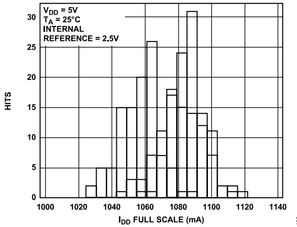
Figure 24. I_{DD} Histogram with Internal Reference, V_{REF} = 2.5 V, Gain = 2
