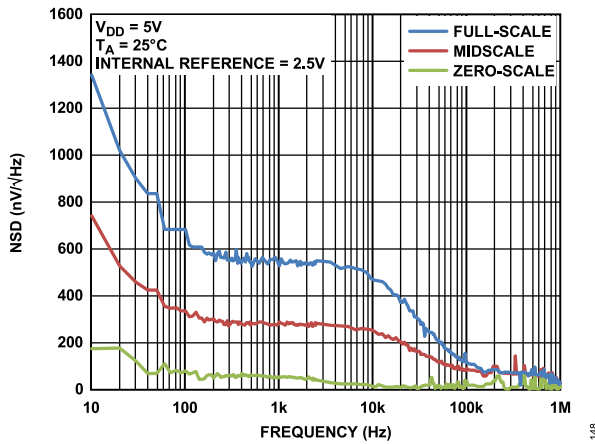
Figure 36. NSD
