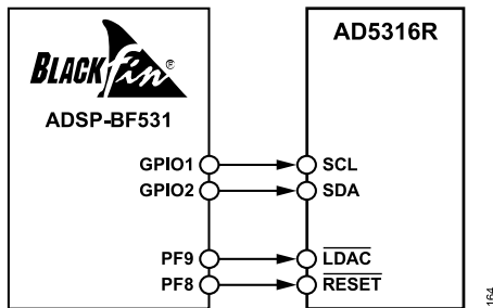
Figure 49. AD5316R to ADSP-BF531 Interface
