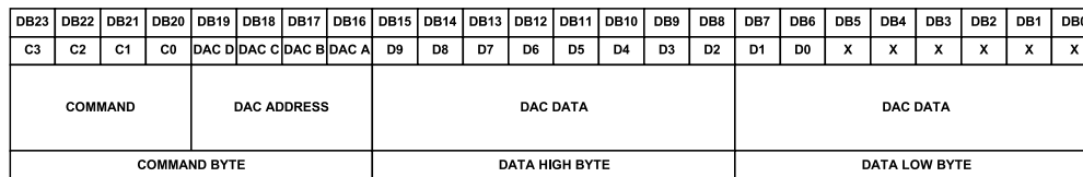
Figure 41. Input Shift Register Contents
