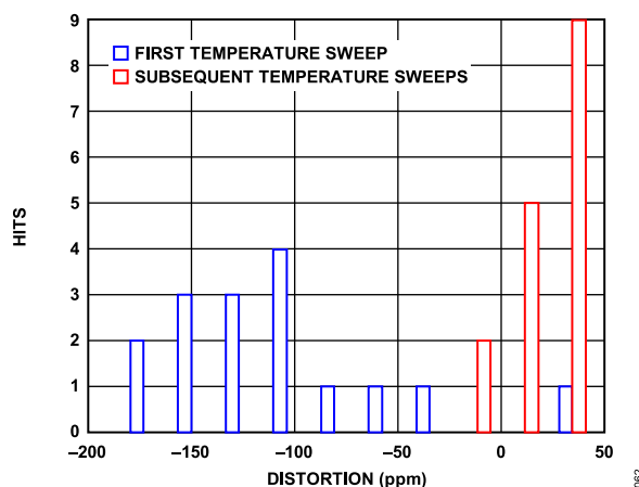
Figure 48. Thermal Hysteresis
