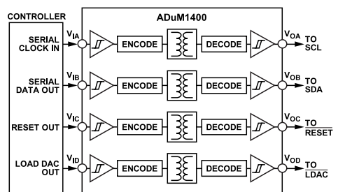
Figure 51. Isolated Interface
