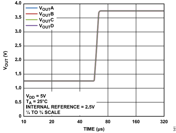
Figure 29. Settling Time
