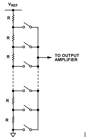
Figure 40. Resistor String Structure
