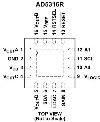
Figure 3. 16-Lead LFCSP Pin Configuration
