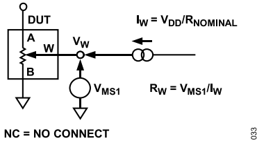
Figure 33. Wiper Resistance
