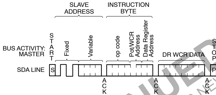
Figure 7. Write Timing
