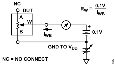
Figure 37. Wiper Resistance
