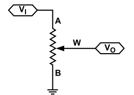
Figure 48. Potentiometer Mode Configuration
