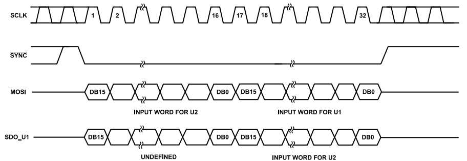
Figure 41. Daisy-Chain Diagram
