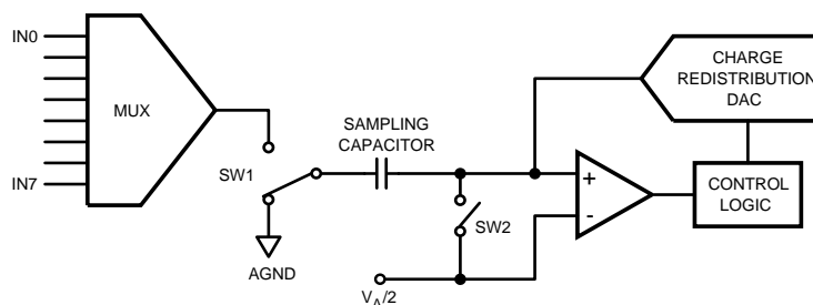
Figure 35. ADC088S052 in Hold Mode
